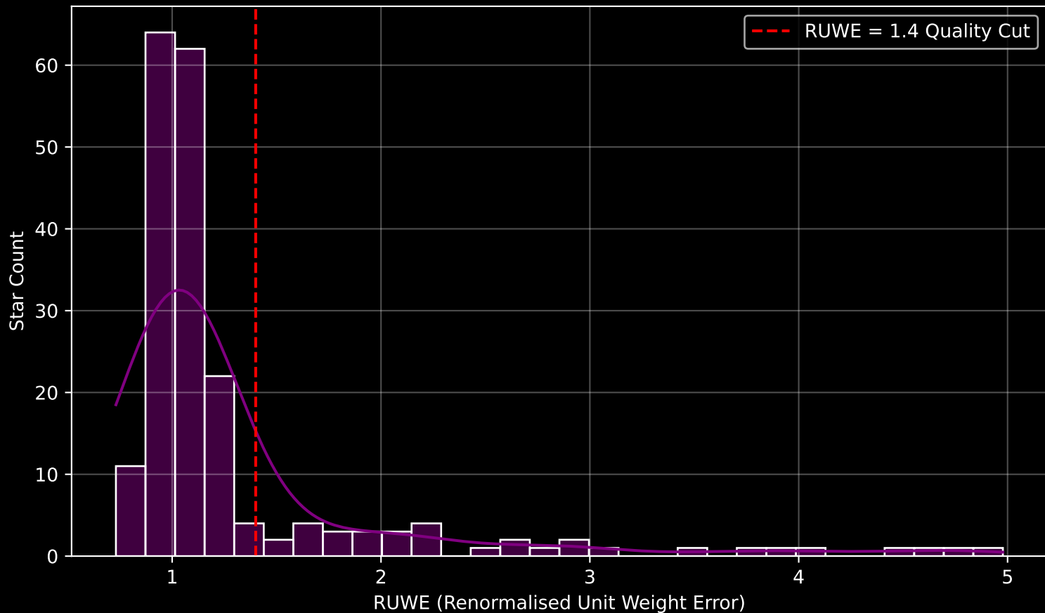
GAPOGEE DR17 Field [154-59_MGA] RUWE Distribution (n= 197)
