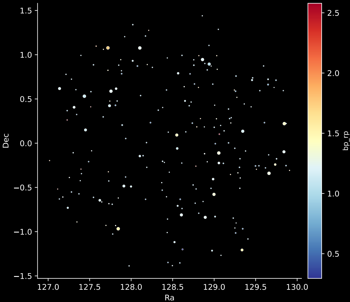
APOGEE DR17 Field: [154-59_MGA] Stars: 206
