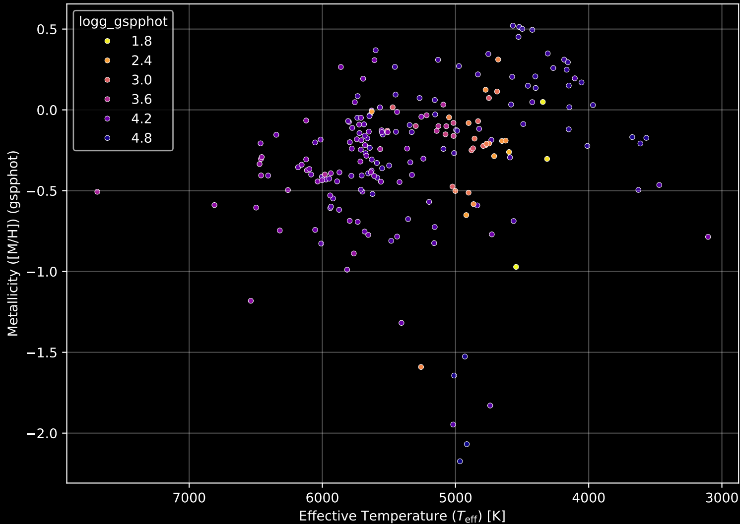
APOGEE DR17 Field: [154-59_MGA] Stellar Population Parameters (n= 206)
