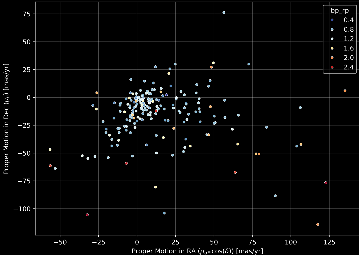
APOGEE DR17 Field: [154-59_MGA] Proper Motion Diagram (n= 206)
