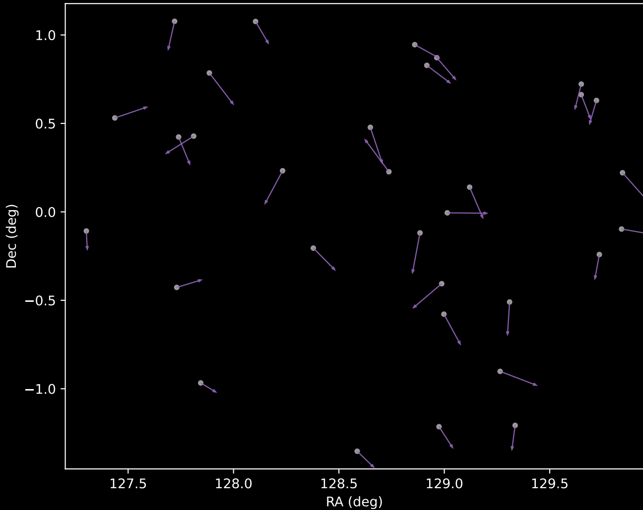
APOGEE DR17 Cluster 8 Proper Motion Vectors (n=32)
