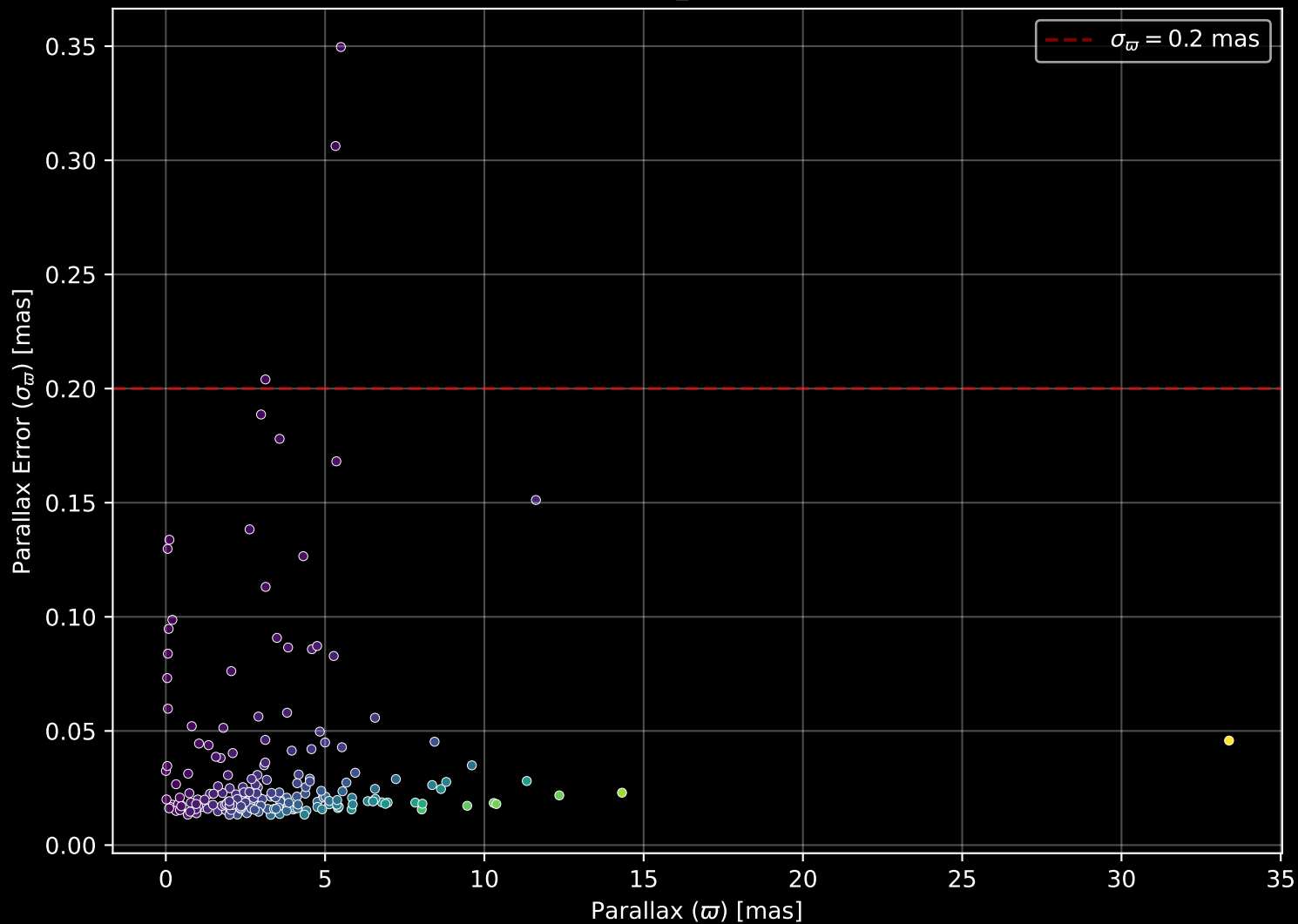
APOGEE DR17 Field: [154-59_MGA] Parallax Quality (n= 206)
