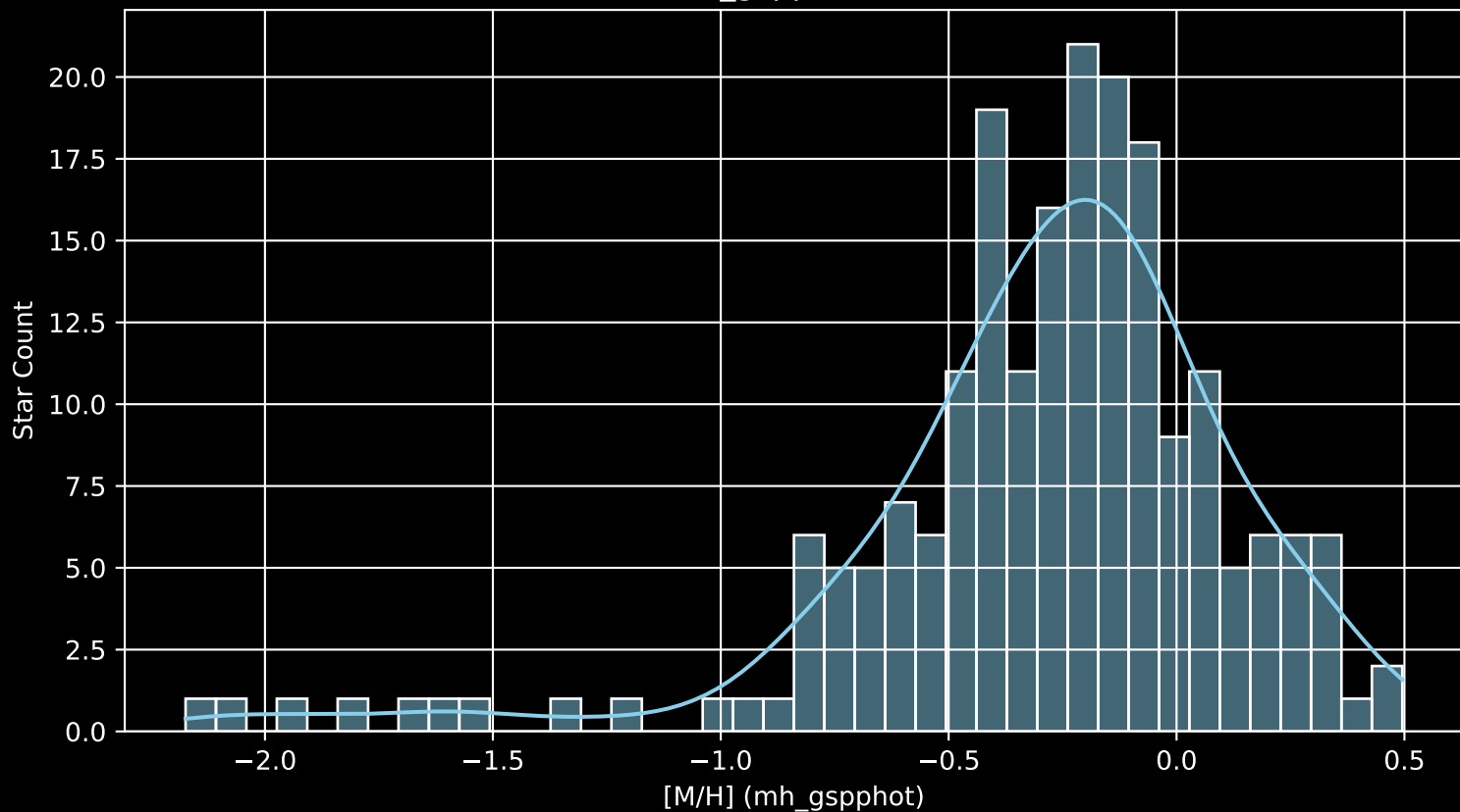
APOGEE DR17 Field: [154-59_MGA [M/H] (mh_gspphot) (n= 203)
